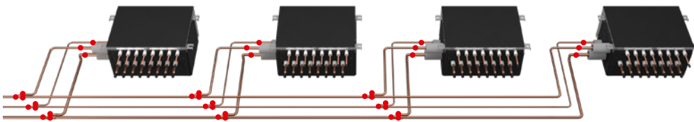
VRV IV: 39 brazing points and 3 joint kits
