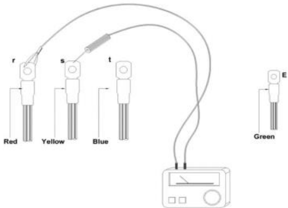
INSULATION RESISTANCE TESTER
