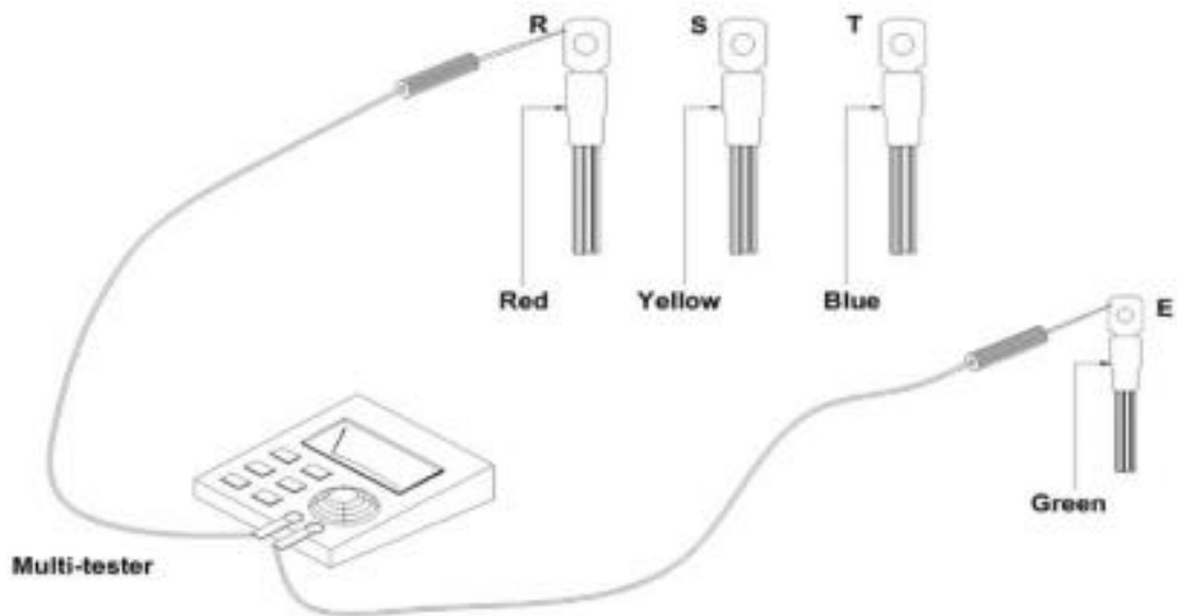
CONTINUITY TEST
